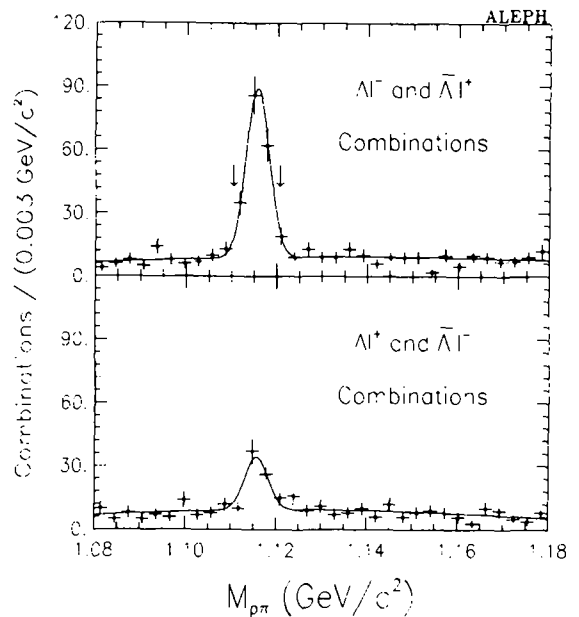
Fig. 1. The p\pi^- invariant mass distribution of the \Lambda\ell^- and \Lambda\ell^+ combinations. Arrows indicate the region used for the \Lambda_b lifetime analysis.
