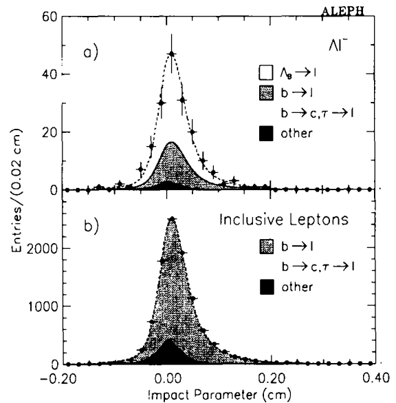
Fig. 2. Lepton impact parameter distributions for the (a) \Lambda\ell^- sample and (b) inclusive lepton sample, together with the results of the unbinned maximum likelihood fits.
